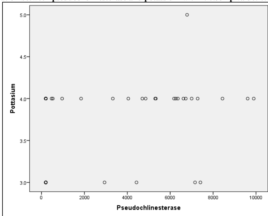
Graph 1: Correlation between pseudocholinesterase and potassium with r: 0.334 p value: 0.027
