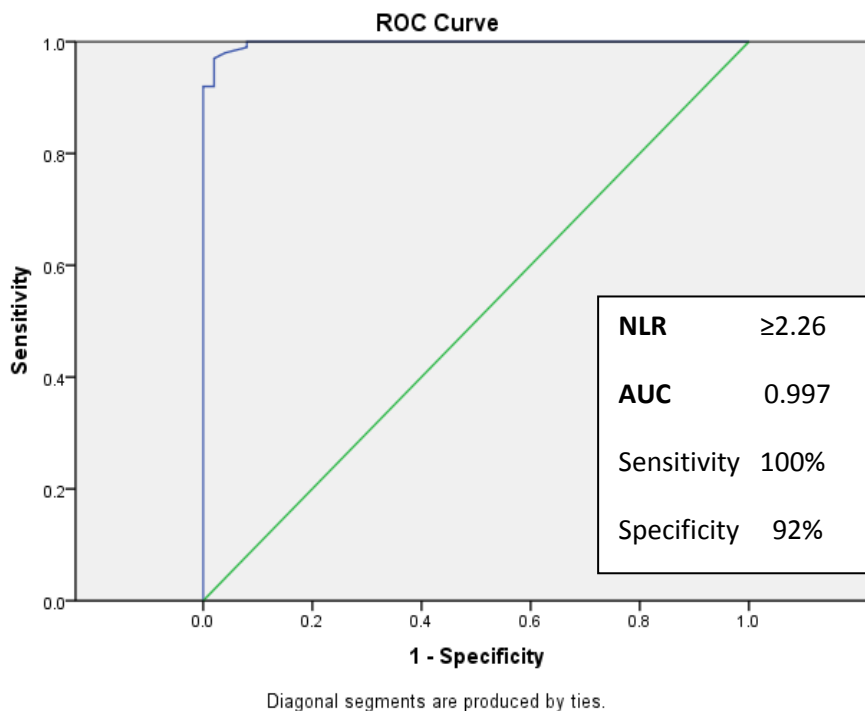
Fig. 1: Receiver- operating characteristic (ROC) curve analysis of NLR for predicting coronary artery disease (CAD) in CAD (+) and CAD (-) in diabetic patients
